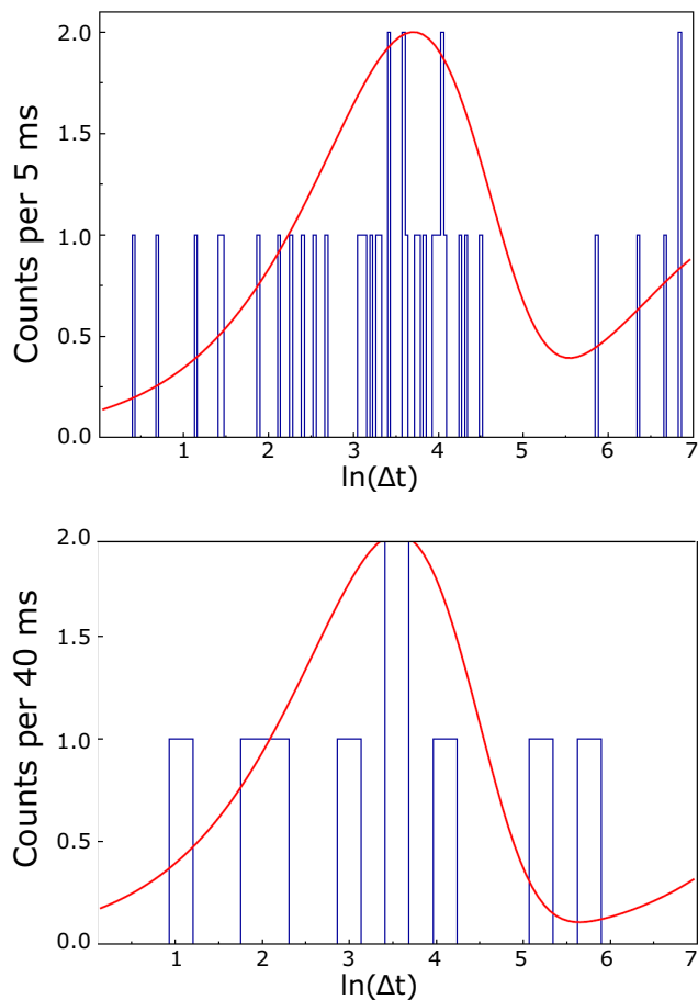
FIG. 5. Natural logarithm, \ln(\Delta t) , showing the time distribution of the correlated \beta -decay WAS3Bi events following the identification of ^{73}\text{Sr} nuclei (top) and ^{76}\text{Y} (bottom) events in BigRIPS. \Delta t is the time difference in ms between detection of the recoils and the \beta^+ events. The solid red curves show the best fit using the Schmidt method to extract the mean lifetimes. These were converted to half-life values of 28_{-4}^{+5} ms for ^{73}\text{Sr} (top) and 24_{-6}^{+12} ms for ^{76}\text{Y} (bottom), respectively. Note: The red curves have been multiplied by a factor to make them visible (the areas under the curve and in the data are not the same).
